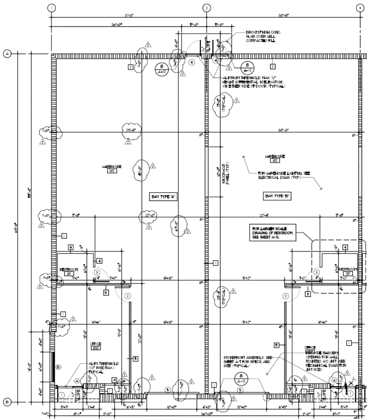
Bay Type 'A' and 'B' Floor Plan 3/16'
