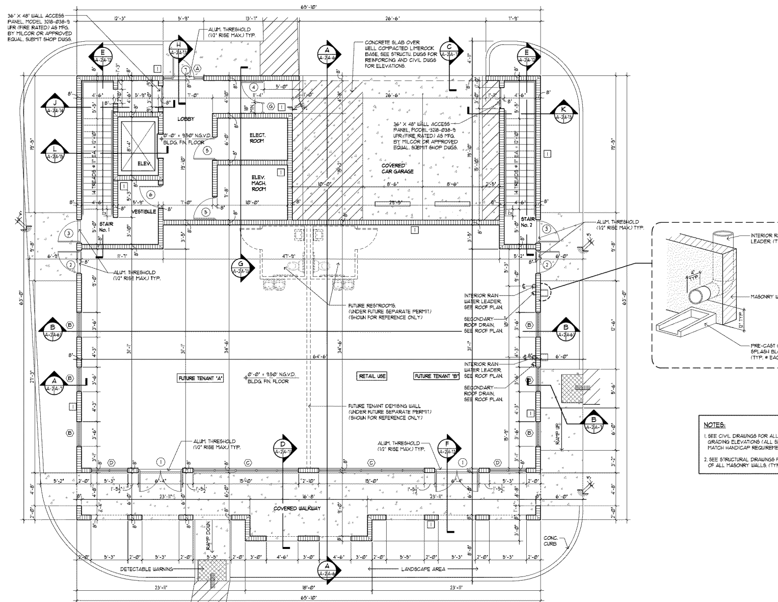
Ground Floor Plan 3/16"
