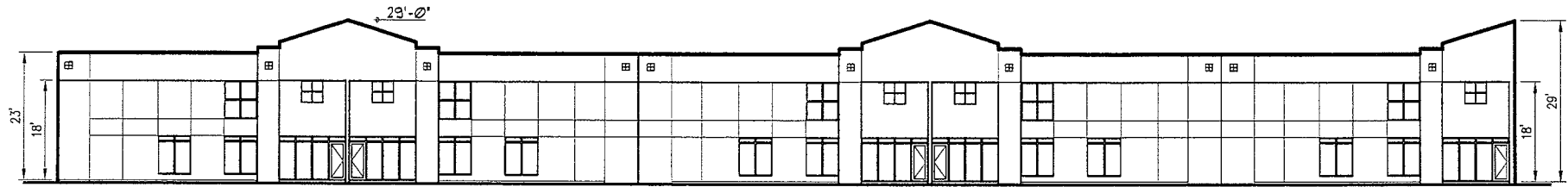
FRONT ELEVATION BUILDING "A & C" BUILDING "B & D" (REVERSED)
