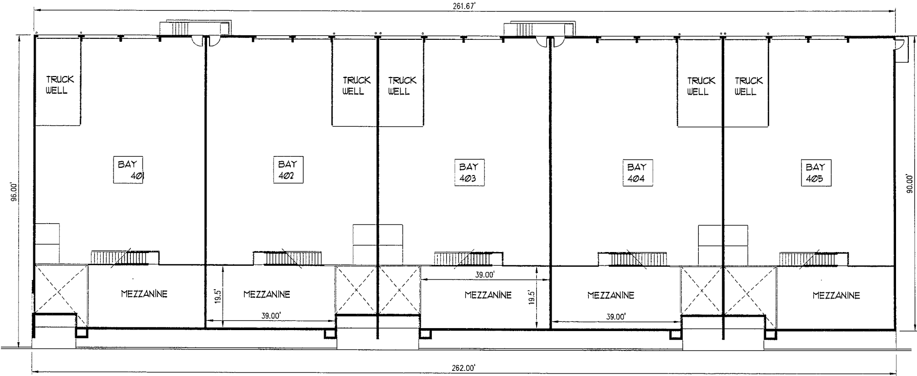
MEZZANINE FLOOR PLAN
