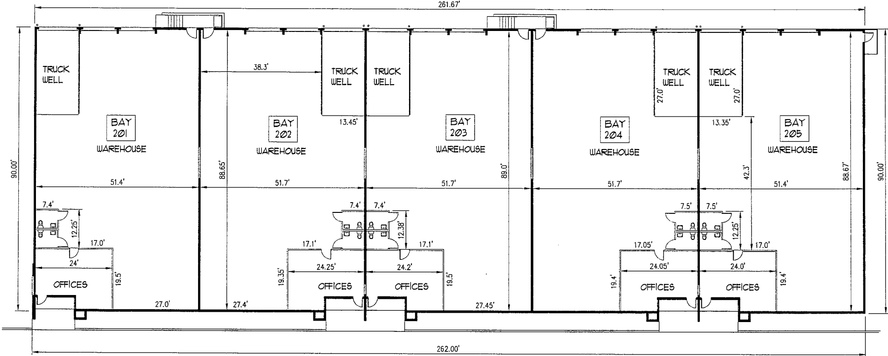
BUILDING FLOOR PLAN
