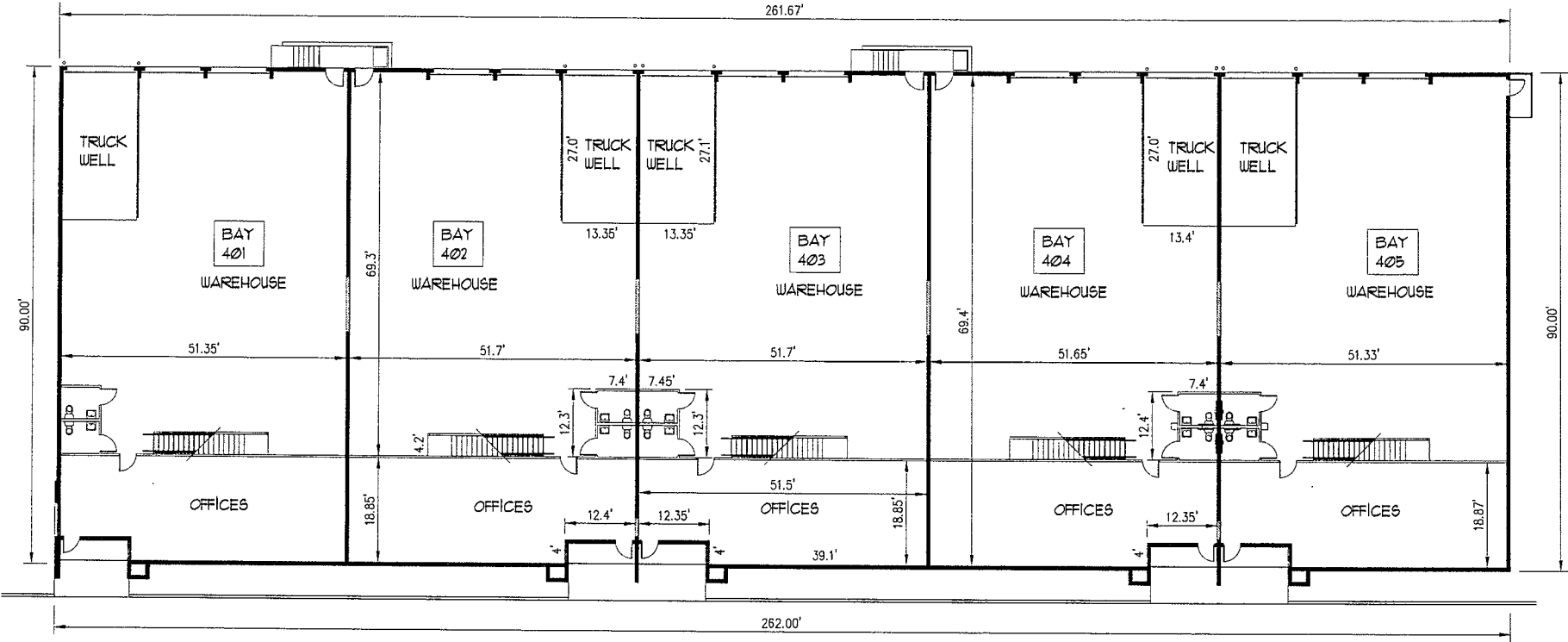
BUILDING FLOOR PLAN
